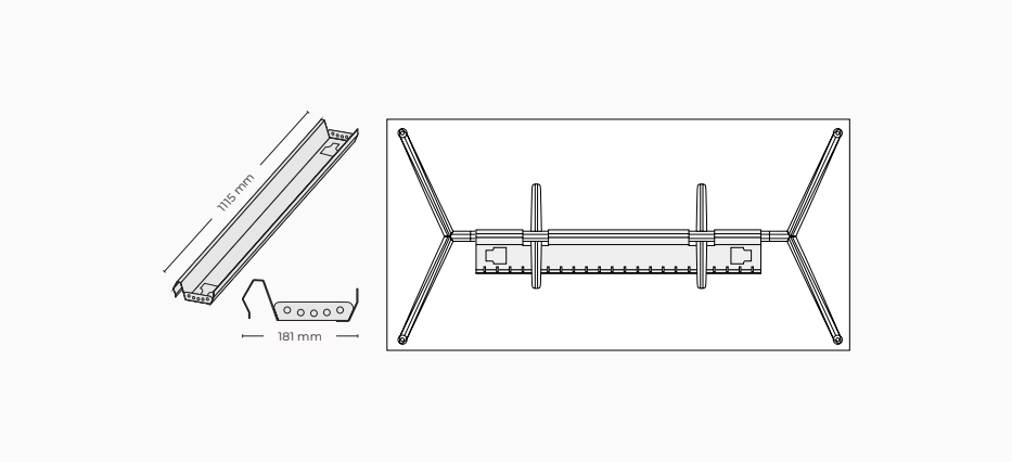
Individual 1150 mm steel tray for individual 1800 and 2000 mm tables.
