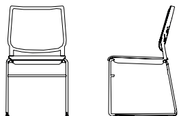
VB13C | Sled Base Uph. Seat & Back.
