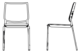
VB17C | 4 Leg Base Uph. Seat & Back.
